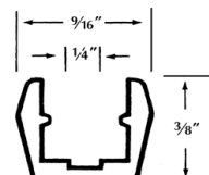
TRACK PROFILE
